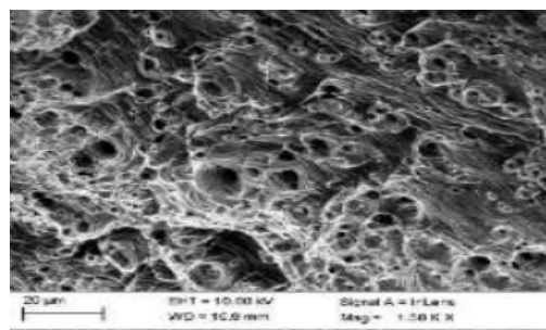
Figure: SEM image of ultimate tensile strength sample Al6061 and 15% of TiB 2
