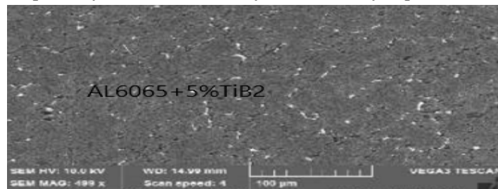
Figure: Micro structure of Al6061 and 5% of TiB 2
