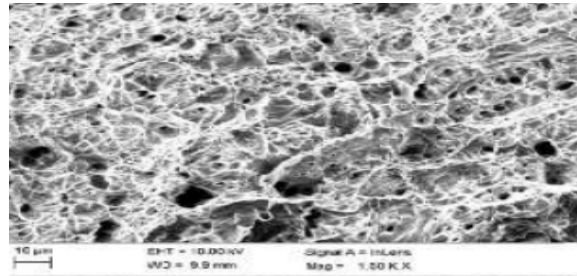
Figure: SEM image of ultimate tensile strength sample Al6061 and 5% of TiB 2
