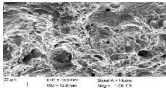
Figure: SEM image of ultimate tensile strength sample Al6061 and 10% of TiB 2
