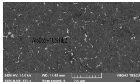
Figure: Micro structure of Al6061 and 10% of TiB 2
